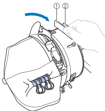
① Handle ② Lever
