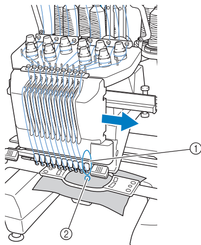
① Needle at the embroidering position The needle is positioned over the hole in the needle plate ②.
