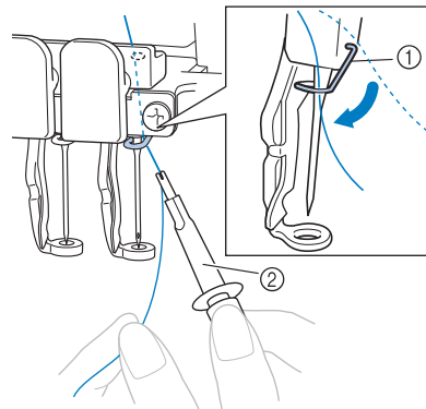
① Needle bar thread guide ② Needle changing tool (Threader)
