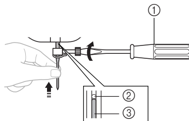
① Screwdriver / Destornillador ② Needle Stopper / Tope de la aguja ③ Needle / Aguja
