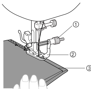
① Screw / Tornillo ② Guide / Guía ③ Folded hem / Dobladillo
